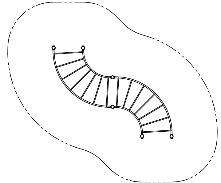
PLAN VIEW WITH USE ZONE SCALE: 1/8"=1'-0"
