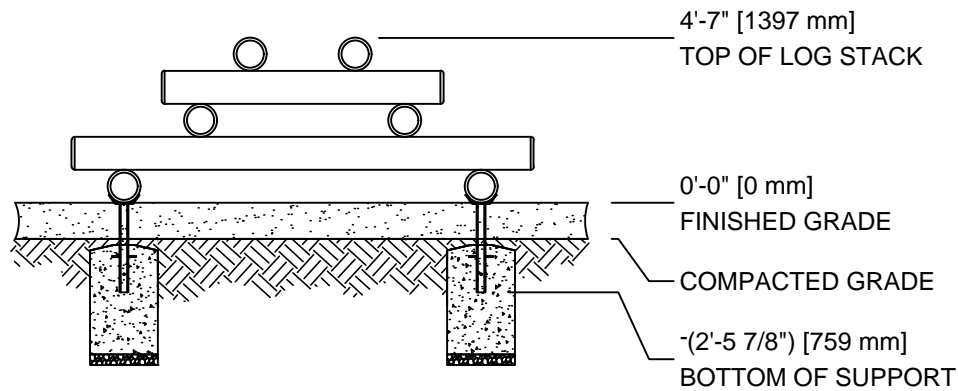
FRONT VIEW SCALE 3/16"=1'-0"
