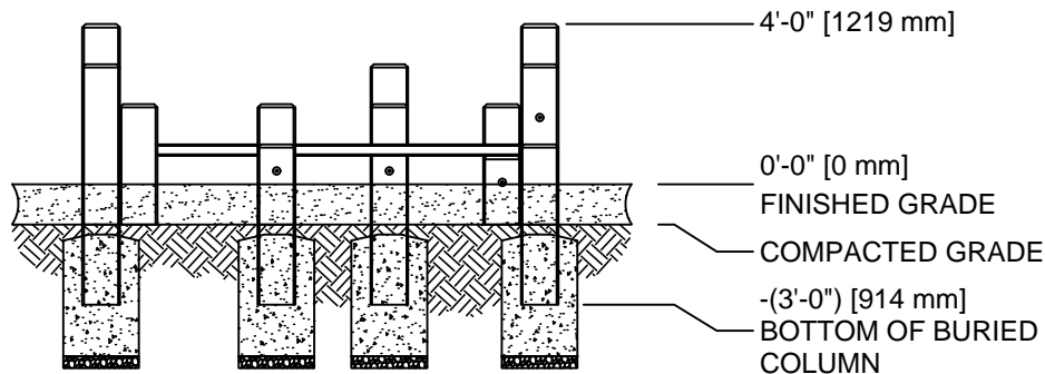
FRONT VIEW SCALE 3/16"=1'-0"
