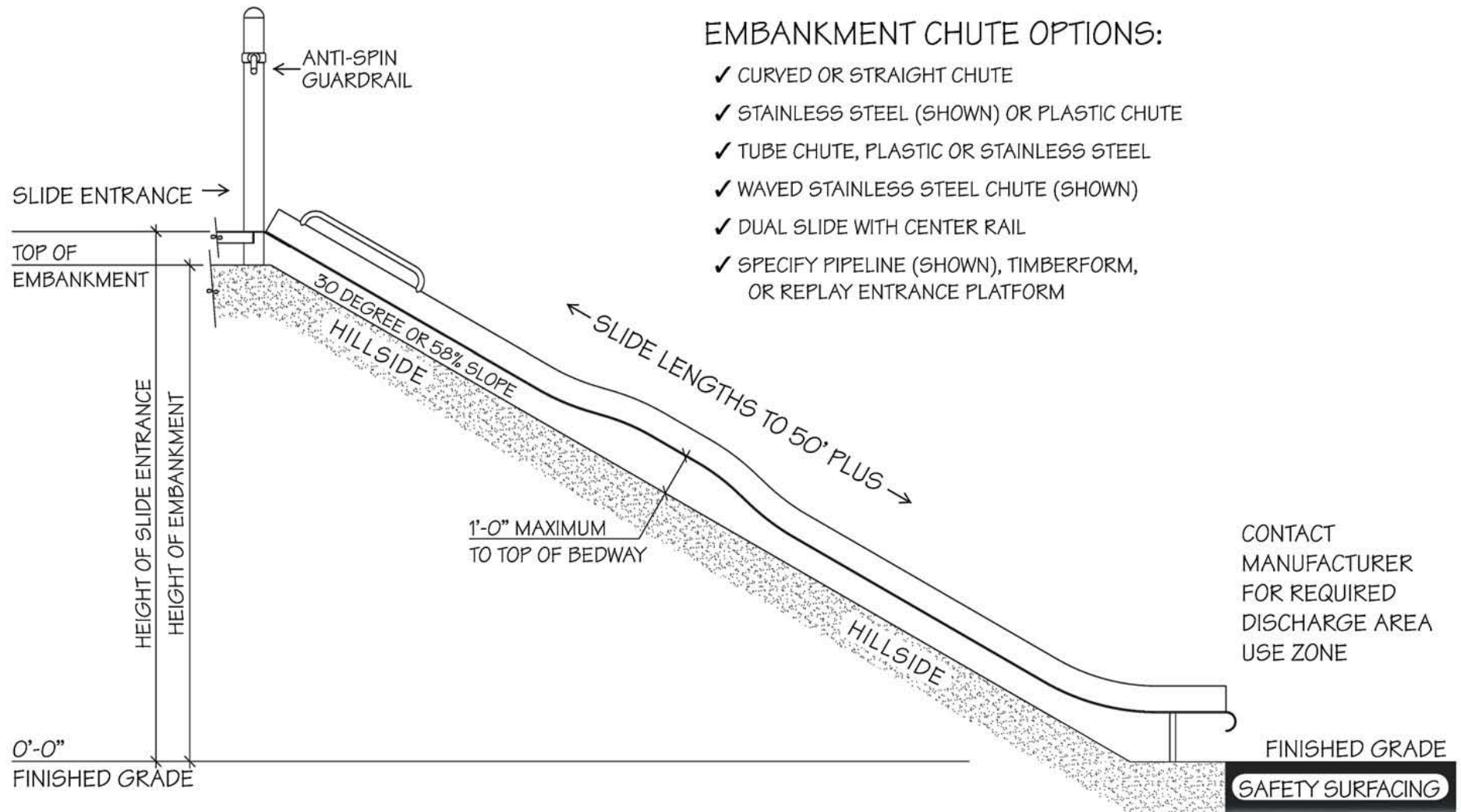
TYPICAL EMBANKMENT SLIDE CHUTE— SIDE VIEW
