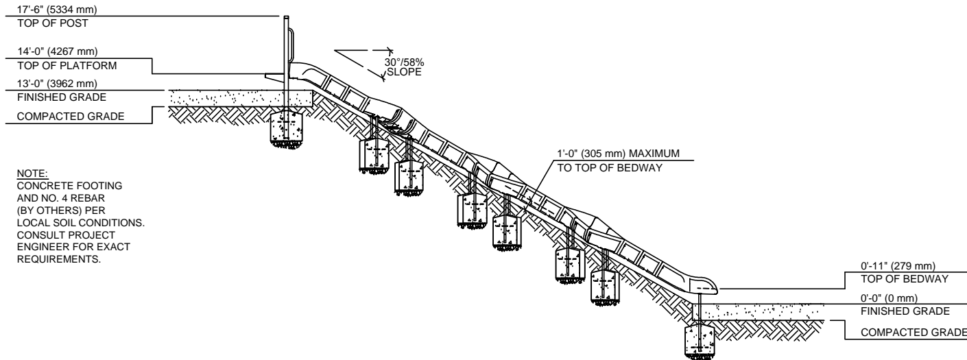
SIDE ELEVATION
