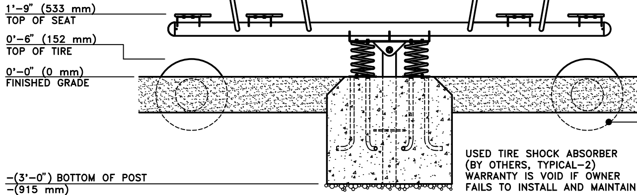
FRONT VIEW SCALE: 3/8"=1'-0"
