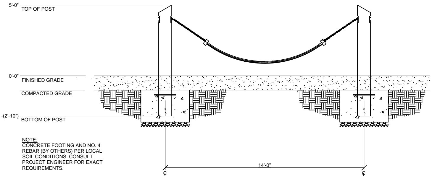
ELEVATION VIEW SCALE 1/4"=1'-0"
