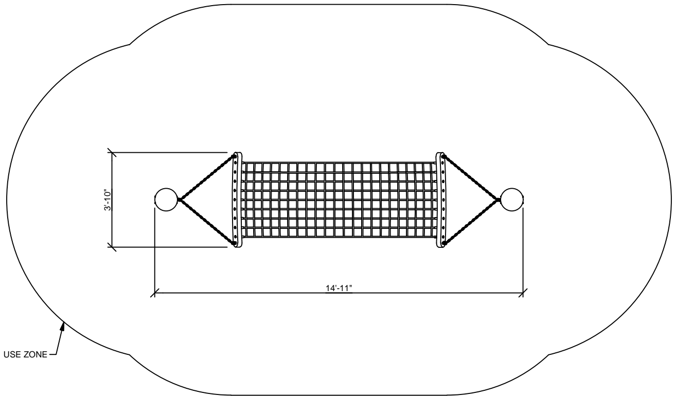
TOP VIEW SCALE 1/4"=1'-0"
