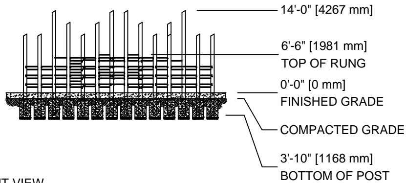
FRONT VIEW SCALE 1/16"=1'-0"
