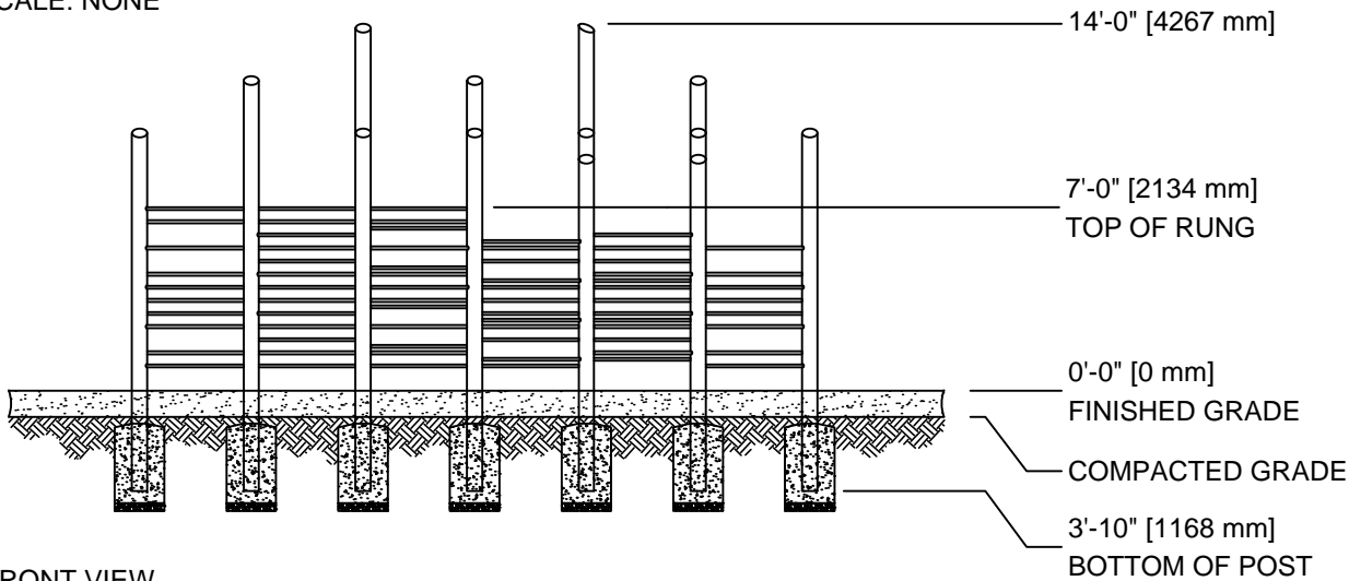
FRONT VIEW SCALE 1/8"=1'-0"
