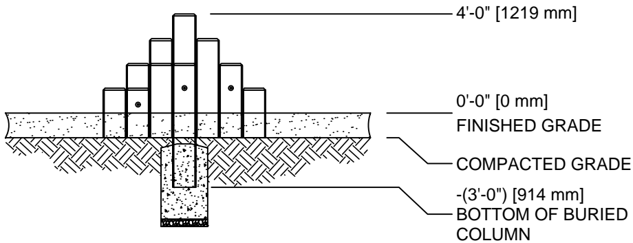
FRONT VIEW SCALE 3/16"=1'-0"
