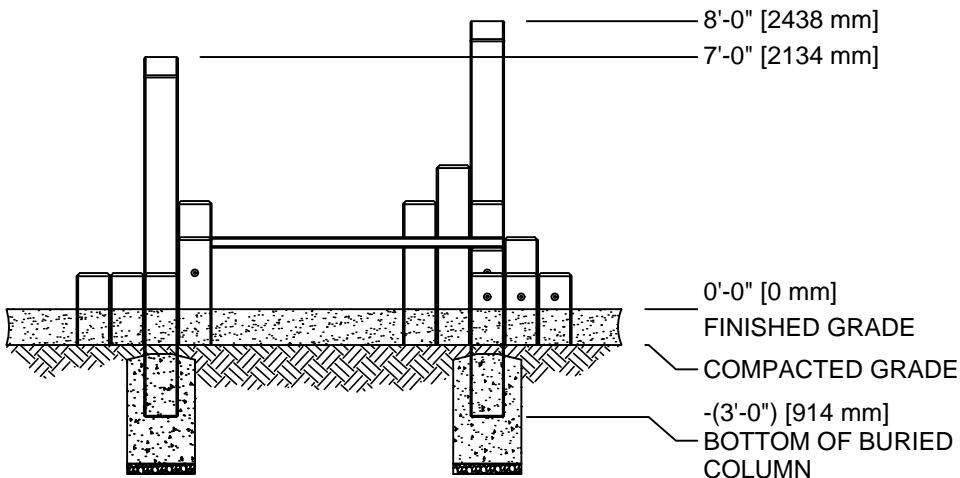
FRONT VIEW SCALE 3/16"=1'-0"
