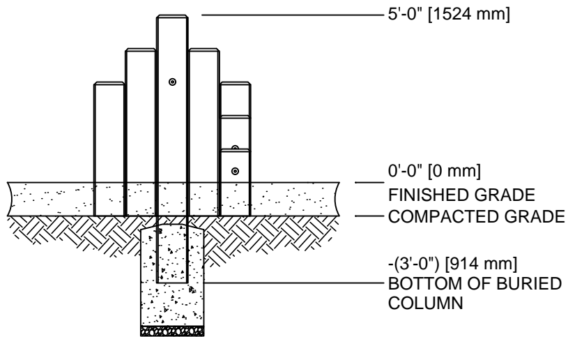
FRONT VIEW SCALE 1/4"=1'-0"
