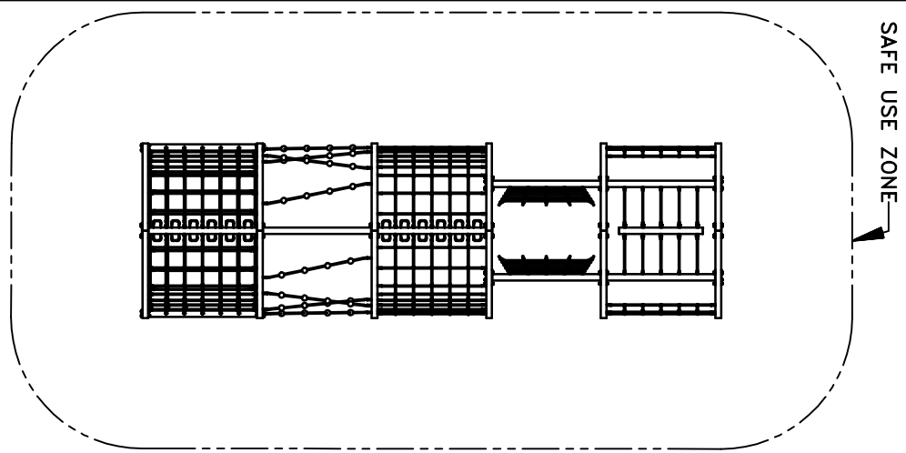
PLAN VIEW WITH USE ZONE SCALE: 1/8"=1'-0"
